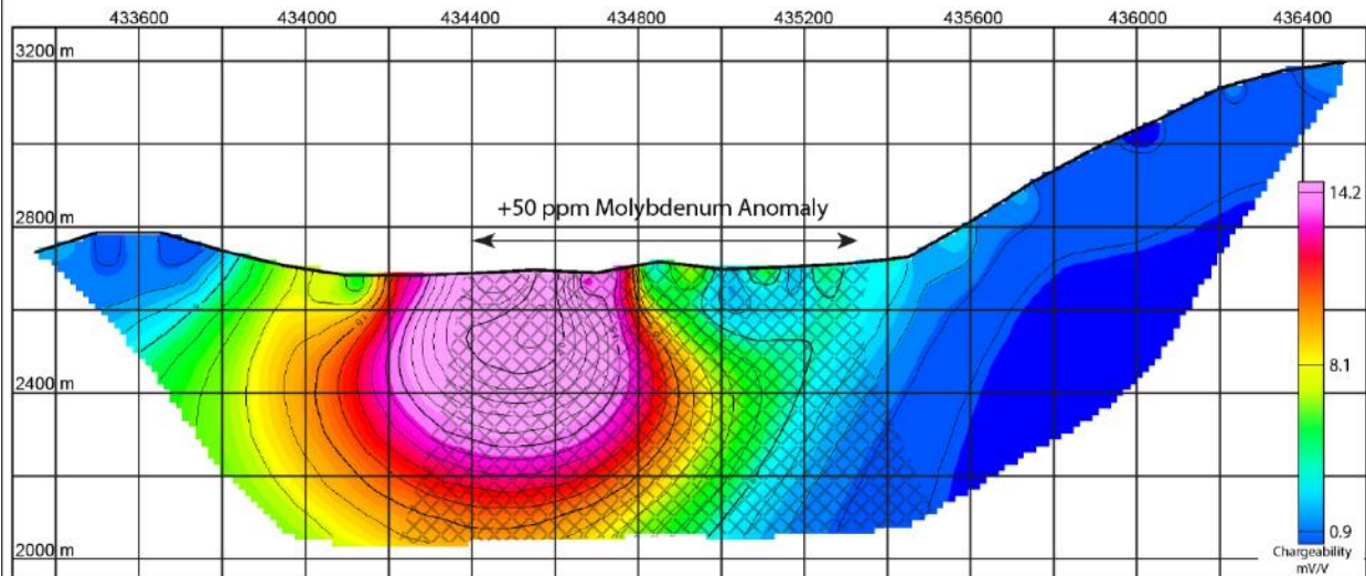
Chargeability Inversion - Line 6960050 N
