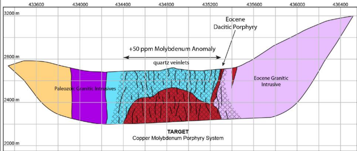
Schematic Geological Cross Section - Line 6960050 N
